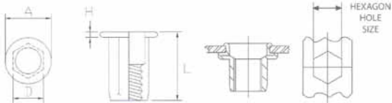
FULL-HEXAGON WITH BIG FLANGE BERYNUT FLAT HEAD, ROUND INTERNAL HOLE, OPEN END
