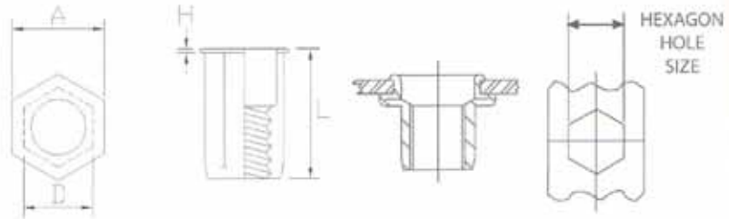
FULL-HEXAGON WITH SMALL FLANGE BERYNUT HEX FLANGE, ROUND INTERNAL HOLE, OPEN END
